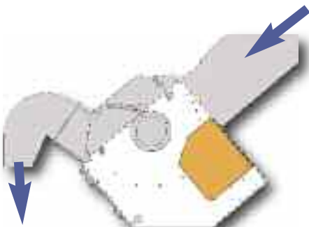
Horizontally fed drum chipper Chip discharge spout at floor level – no need for a pit
