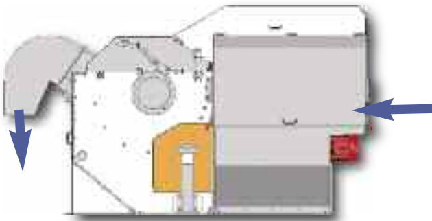
Horizontally fed drum chipper Chip discharge spout at floor level – no need for a pit
